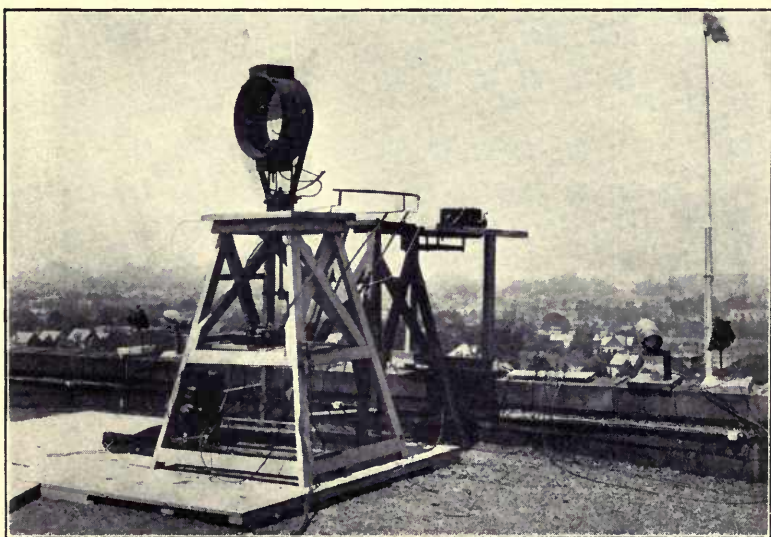
General View of Complete Set-up for the Various Tests on Landing and Signalling Lights
