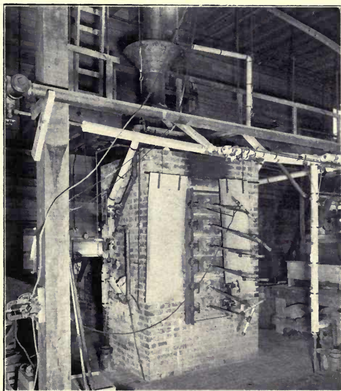
Upper Photo—The small Experimental Electric Furnace Developed for the Steam Activation of Charcoal.
