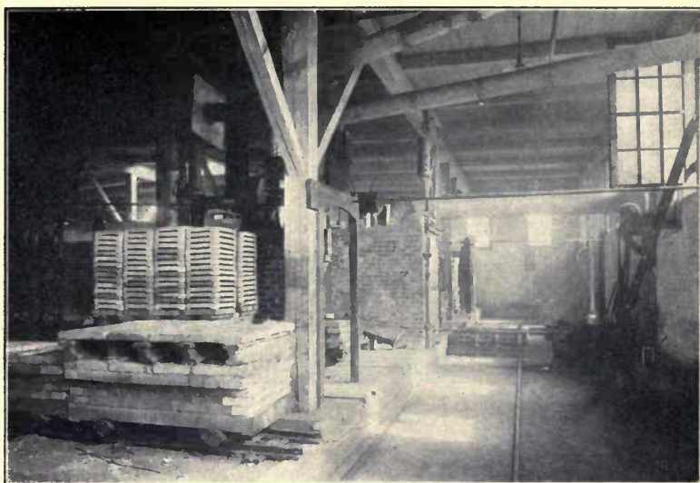
The Charge End of the Tunnel Kiln Type of Furnace. An empty, and a loaded truck are seen in the left foreground
