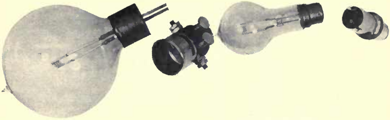
Samples of 33-ampere and 80-ampere 12-volt Projector Lamp developed for use in Combined Landing-and- Searchlight Unit for Airplanes
